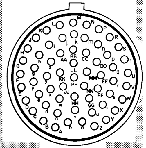
J3-MS3470L24-61PX (FRONT VIEW)
