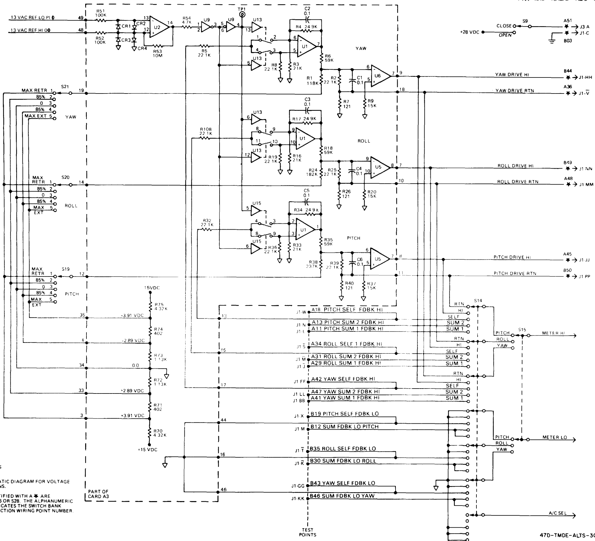
FO-5. Extensible Link Servo-Control Simplified Schematic Diagram
