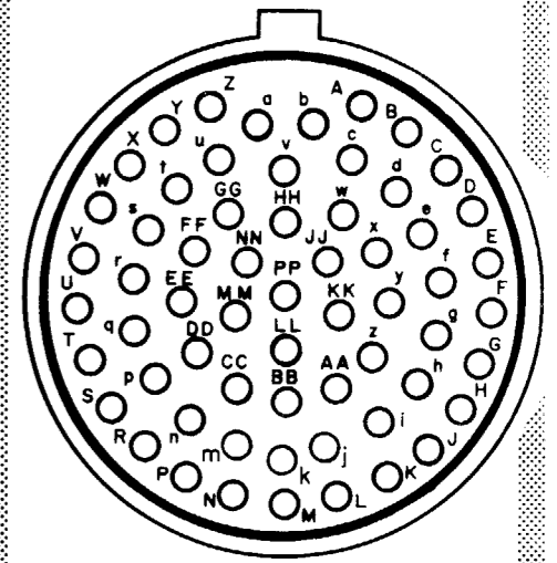
J1-MS3470L24-61P (FRONT VIEW)
