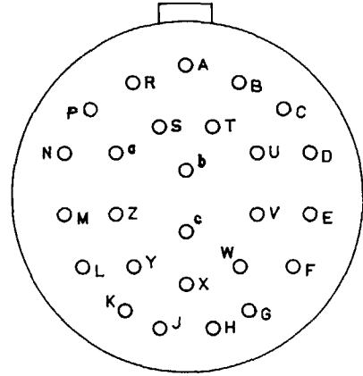
J4 PIN ARRANGEMENT
