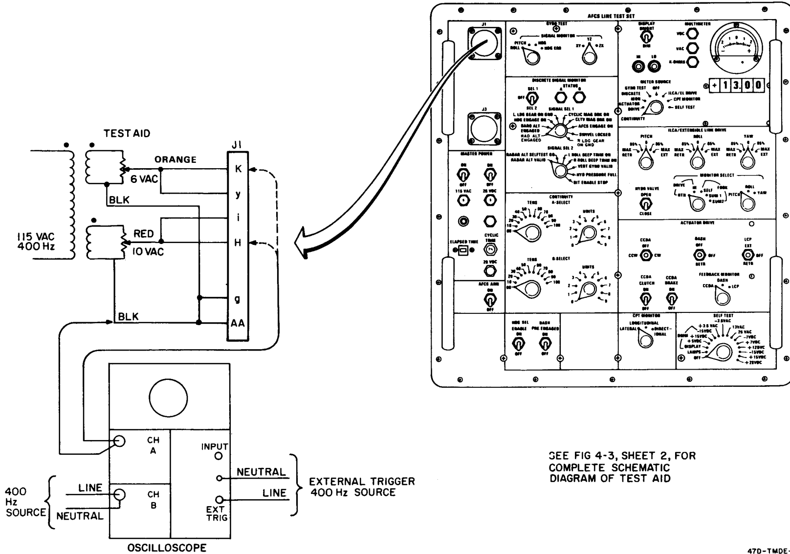
Fig. 4-4. CPT Monitor Test Setup
