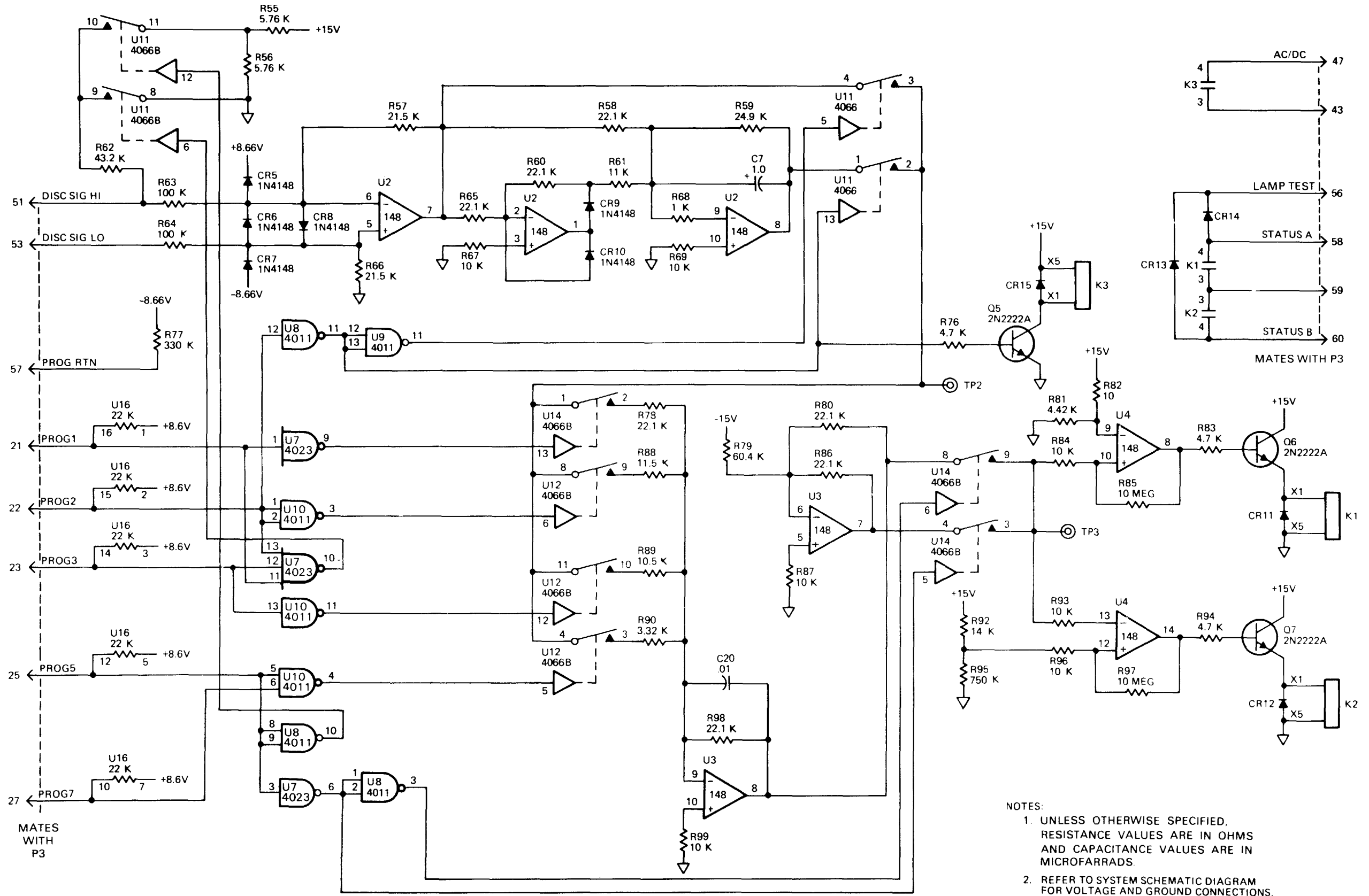
FO-3. Discrete Signal Monitor Detailed Schematic Diagram
