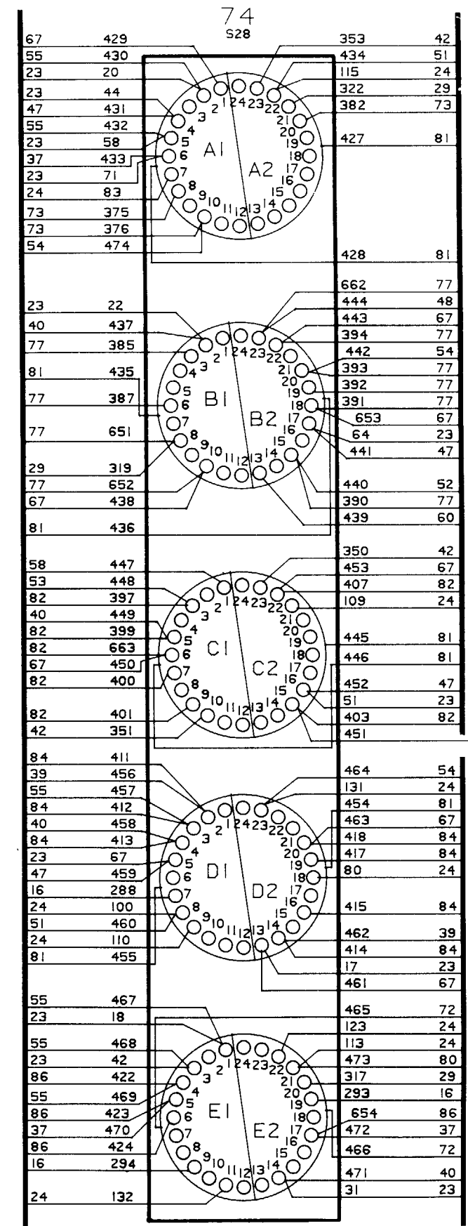
FO-22. Wiring Diagram (Sheet 5 of 5)
